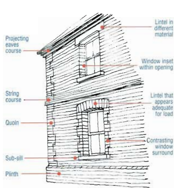
Some common forms of brick detailing Traditionally a more 'humble' building would not have quoins, projecting eaves course, string course, window surround or contrasting brick colours.
